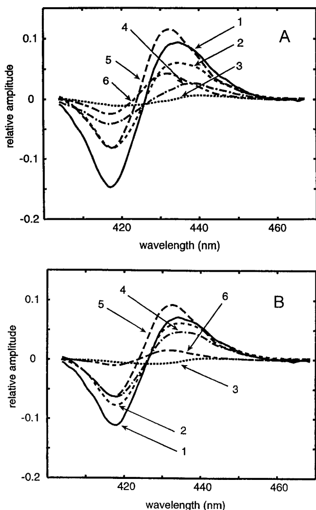
FIGURE 2 Soret band absorbance changes (b-spectra) associated with the time constants reported in Table 1. Relaxations: 1 (—), 2 (---), 3 (· · ·), 4 (— · —), 5 (— · —), and 6 (— · —). (A) PEG-free; (B) 30% PEG-200.
