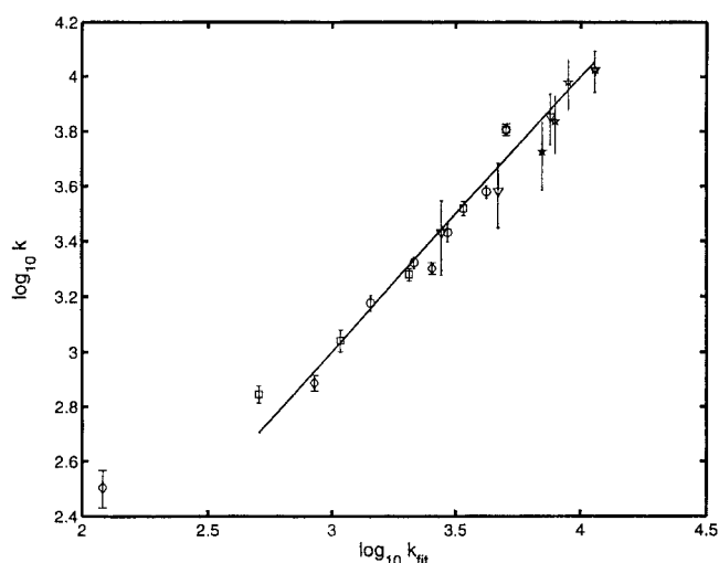
FIGURE 6 Log-log plot of k_{R_0 \rightarrow T_0} calculated from fit to Eq. 22 versus experimental values for HbCO with various cosolutes, using the corresponding fitting parameters in Table 4. PEG-200, 0.1 M phosphate (triangle); cosolute-free pH buffer, ~0.1 M phosphate (star); sucrose, 0.1 M borate, pH 8.3 (open circle); glycerol, 0.1 M borate, pH 8.3 (open square); and ethylene glycol, 0.1 M borate, pH 8.3 (open diamond). PEG-200 and cosolute-free buffer values are from Table 3, where corresponding pH values (7.3–7.9) are tabulated. The values of k and error bars for sucrose, glycerol, and ethylene glycol are taken from Sawicki and Khaleque (1983).
