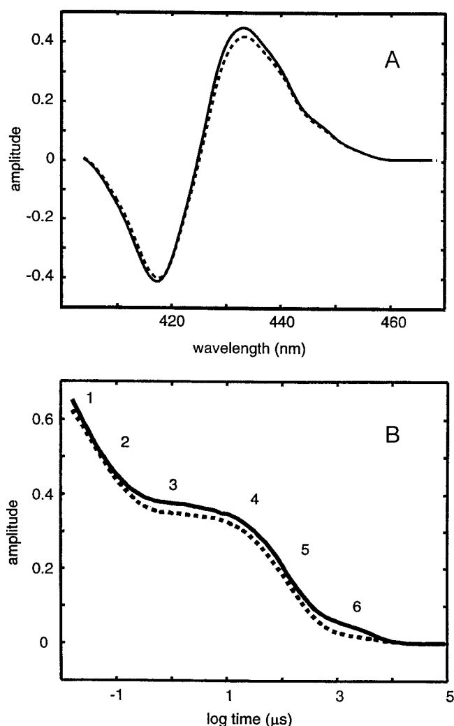
FIGURE 3 First SVD component of the data shown in Fig. 1. (A) Basis spectra ( U_1 ) for PEG-free (solid line) and 30% PEG-200 (dashed line) solutions. (B) Amplitude time courses ( V_1 ), legend as in (A).
